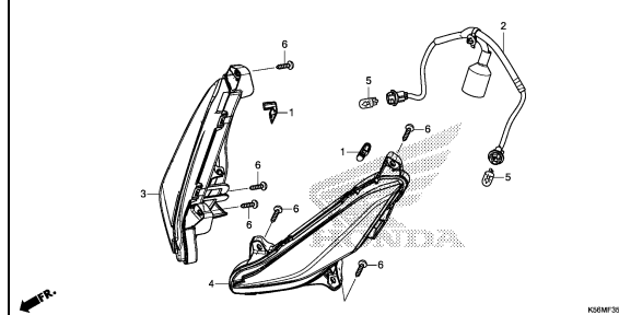
POSITION LIGHT
