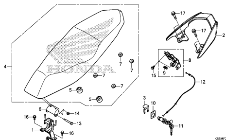
SEAT
