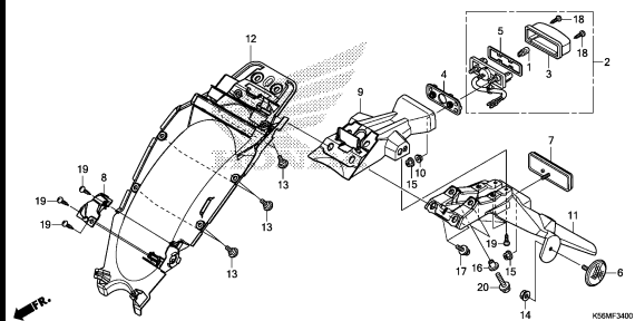
REAR FENDER
