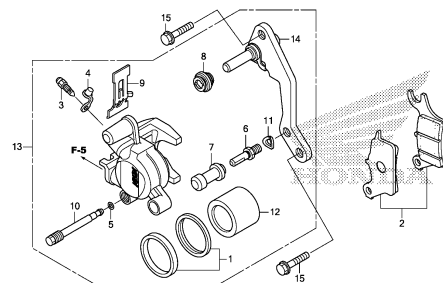
REAR BRAKE CALIPER
