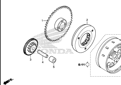
STARTING CLUTCH
