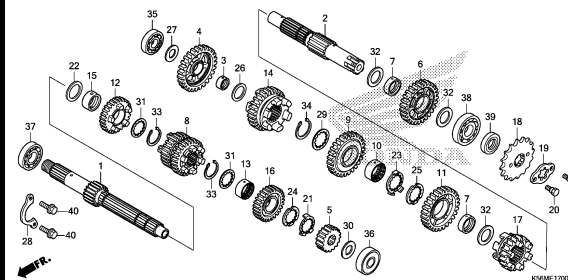
TRANSMISSION
