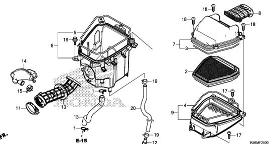
AIR CLEANER
